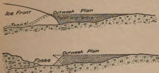
g. 309. — Diagrams to show the manner of formation and the structure of an outwash plain, and the position of the fosse between this and the moraine.
